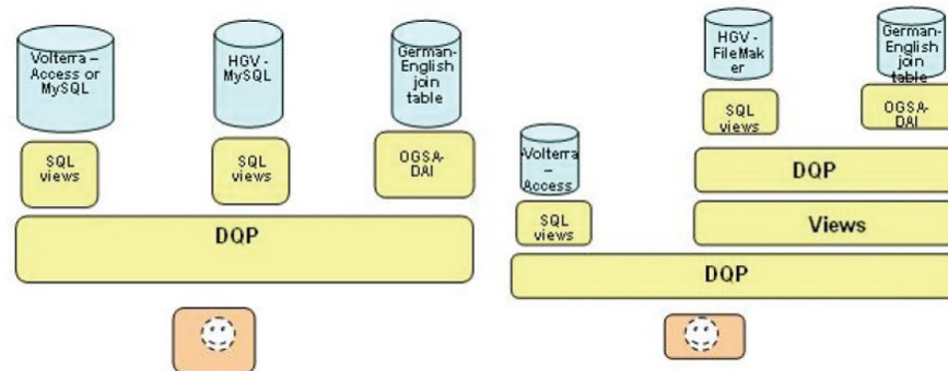
Figure 1: LaQuAT Architecture
