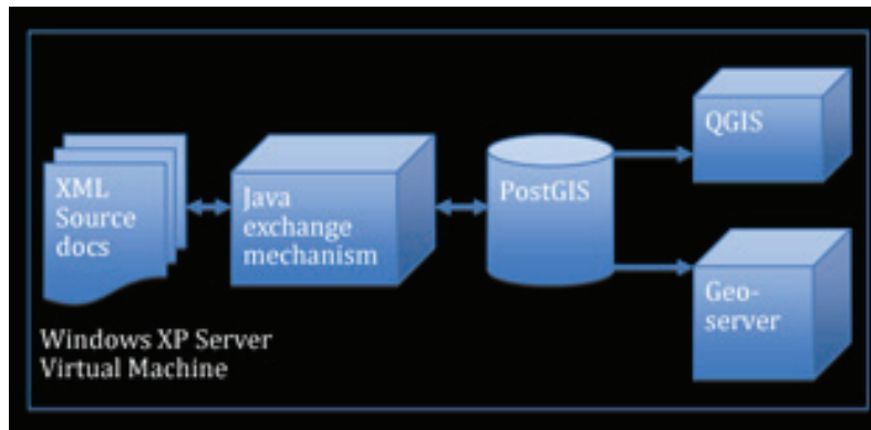
Figure 4: Hestia's architecture
